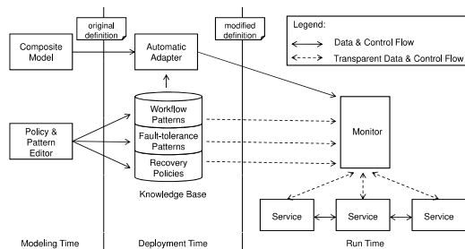
Fig. 3. Conceptual architecture of a reconfigurable composition system
