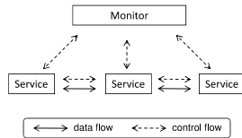
Fig. 2. A hybrid service composition model
