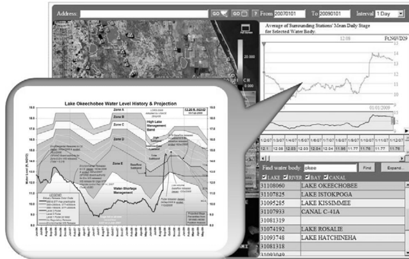
Figure 13. Geospatial-temporal Plots
