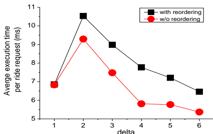
Fig. 19. Time cost of schedule reordering.
