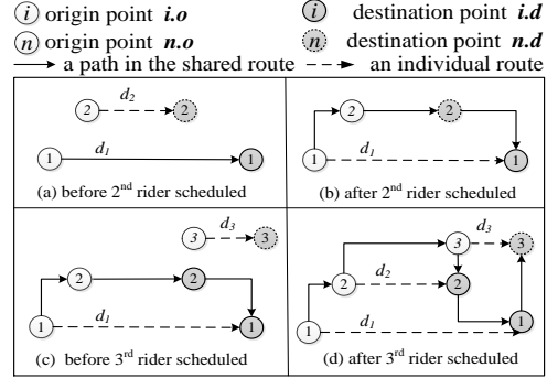
Fig. 12. An example of the pricing constraint.
