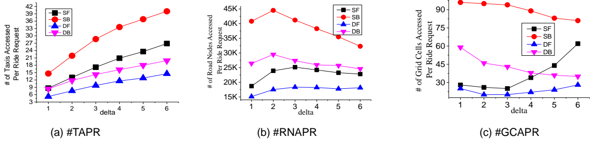
Fig. 18. Computation cost in terms of node access per ride request.
