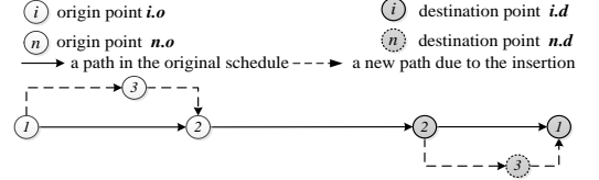
Fig. 11. One possible insertion of a ride request into a schedule.
