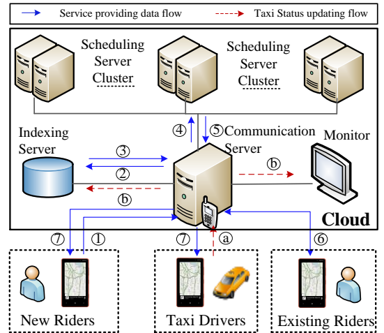
Fig. 1 The architecture of the real-time taxi-sharing system
