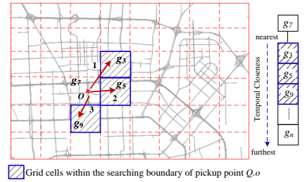
Fig. 7 The single-side taxi searching algorithm
