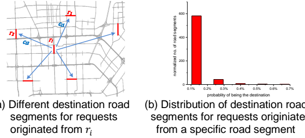
Fig. 14 Transition probability of road segment r_i during a time frame f_j
