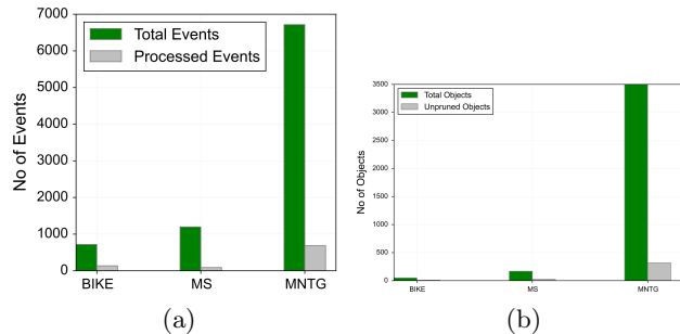
Figure 9: (a) Events Pruning (b) Objects Pruning.
