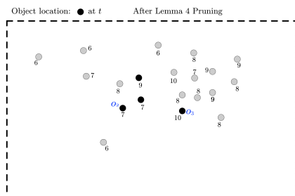
Figure 8: Application of Lemma 4 in \vec{D}O events.
