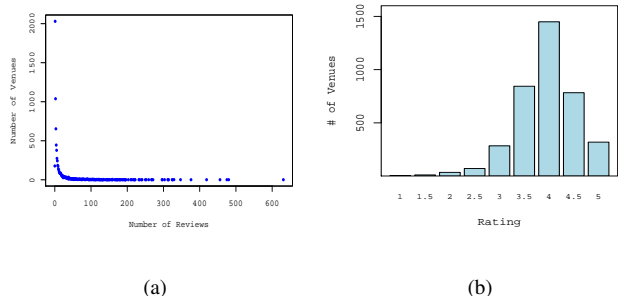
Fig. 1. Statistics of Miami venues: (a) Distribution of number of reviews per venue. (b) Distribution of venue ratings. Venues recording less than 4 reviews were filtered out.
