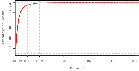
Fig. 7. Safety index values: Distribution of CI values (Crime Index) on blocks in Miami-Dade County.
