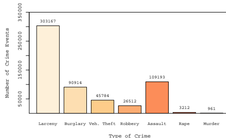
Fig. 2. Outcome of DT classifier – statistics of crime in Miami-Dade county. Distribution of number of crime events per type of crime.
