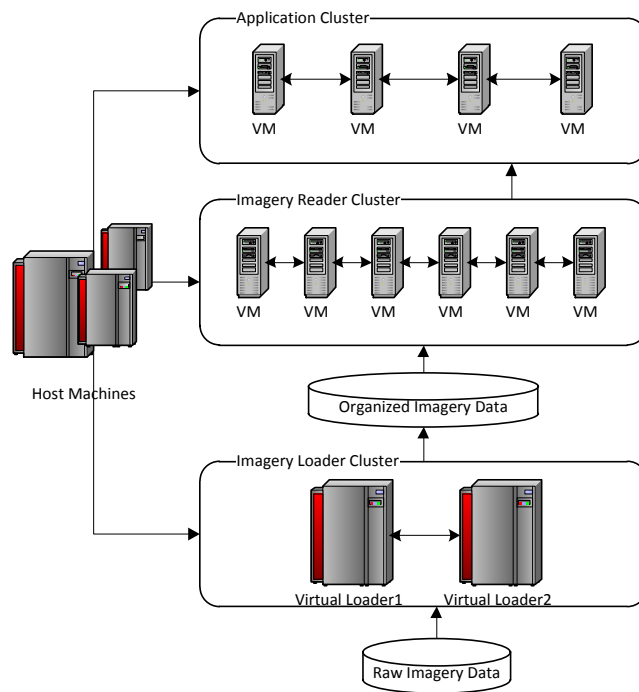
Figure 2: Virtualized TerraFly System
