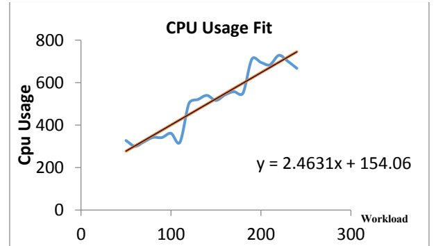
Figure 6: Workload to CPU Usage model
