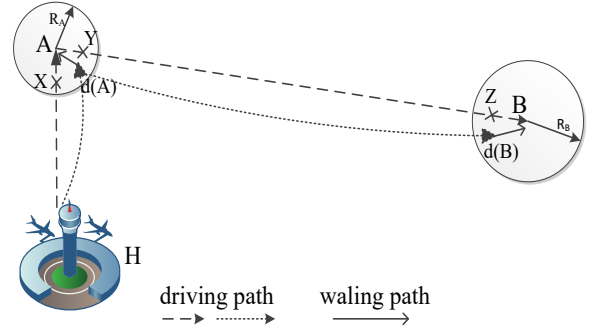
Fig. 3: Demonstration of the proof of Theorem 2
