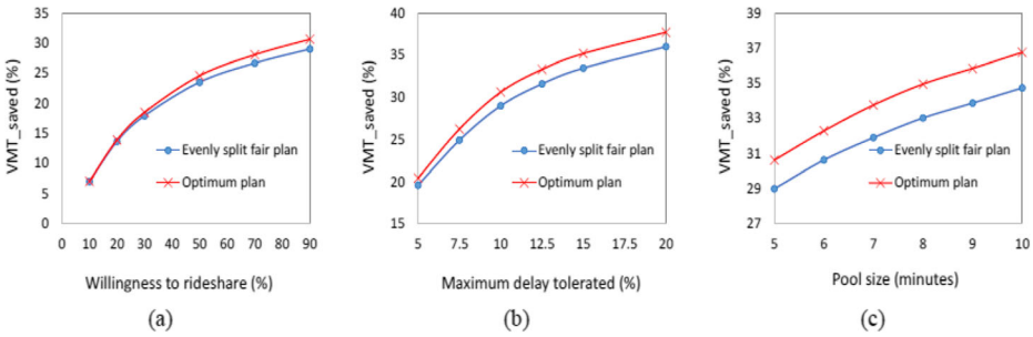
Fig. 4 Static model combining at most two requests: %VMT_saved by the optimum and even-split fair plans
