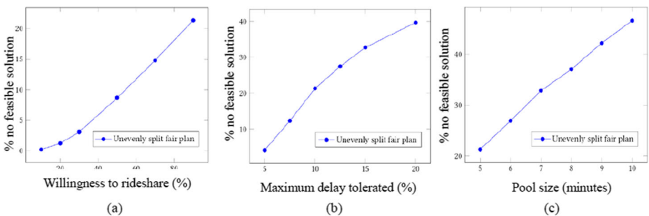
Fig. 7 Static model combining at most two requests: % of pools for which no fair RSP exists with the uneven-split RSG
