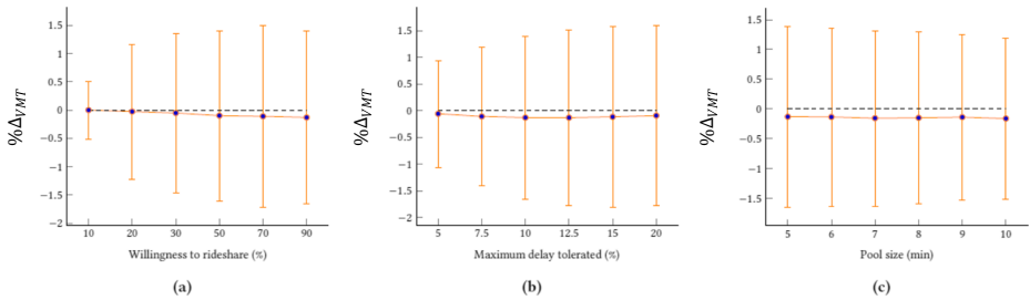
Fig. 6 Static model combining at most two requests: \% \Delta_{VMT} between uneven- and even-split fair plans. The figure gives the average and range of the standard deviation
