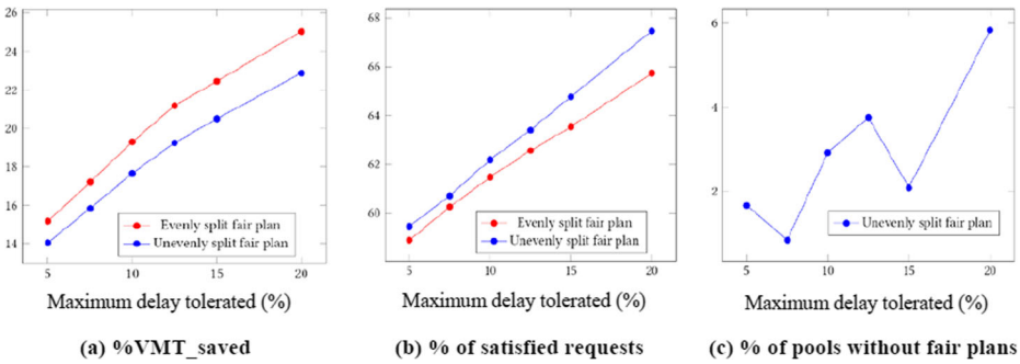
Fig. 11 Dynamic model: comparison between even- and uneven-split fair plans
