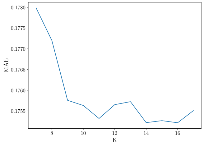
Fig. 5. MAE under different values of K .
