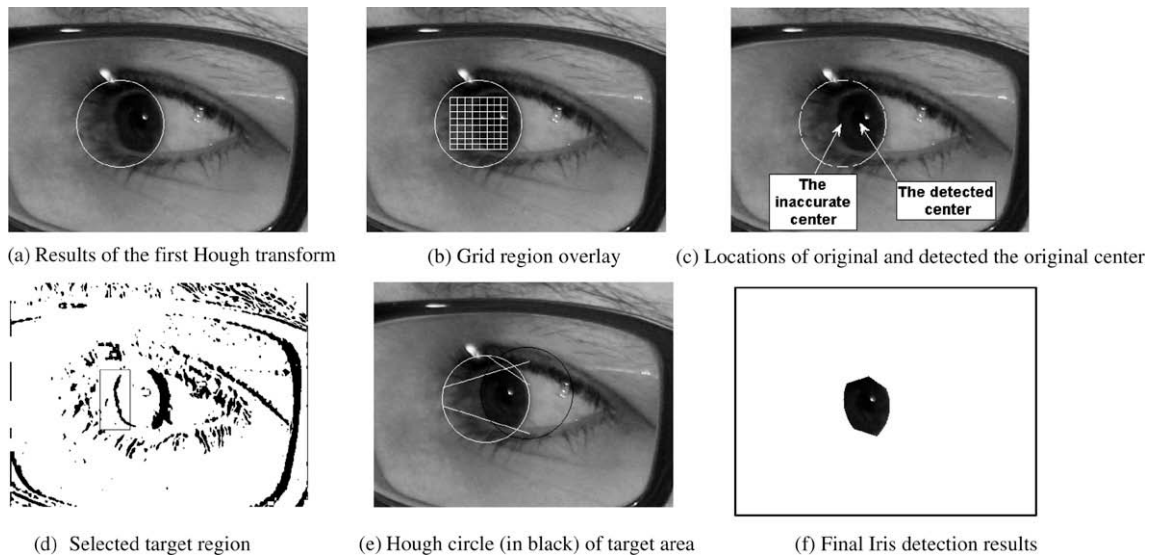
Fig. 10. Defining the non-circular iris boundary – the intersection of the two circles with the detected eyelids lines is the accrual iris.
