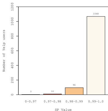
Fig. 12. Distribution of SP values of Yelp users.
