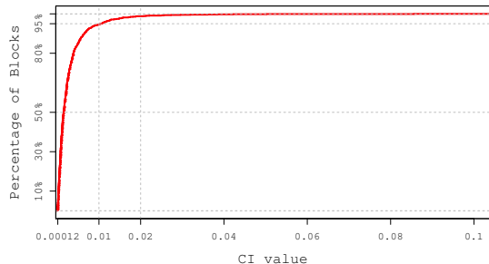
Fig. 11. Safety index values: Distribution of CI values (Crime Index) on blocks in Miami-Dade County.
