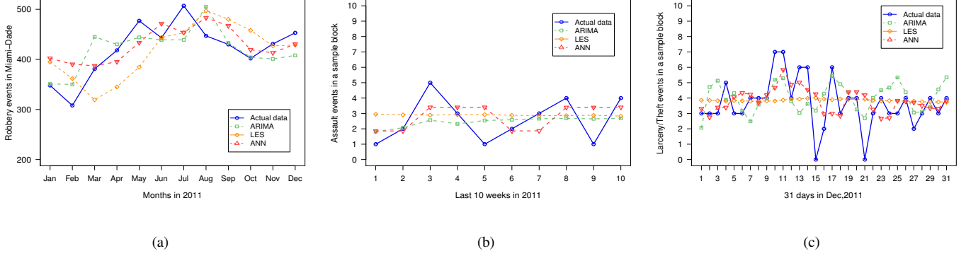
Fig. 5. Crime Forecasting Experiments in Miami-Dade: (a) Prediction of robberies, 2011 monthly basis. (b) Prediction of assaults in a given block for the last 10 weeks of 2011. (c) Prediction of larcenies in a given block for the last 31 days of 2011.
