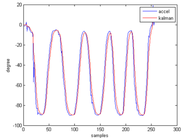
Figure 7: Comparison between Kalman filter output and the accelerometer result
